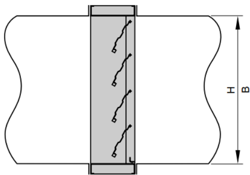
Duct installation
