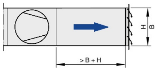
Installation on the discharge side of a fan
